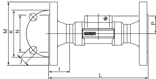
Flange connection
